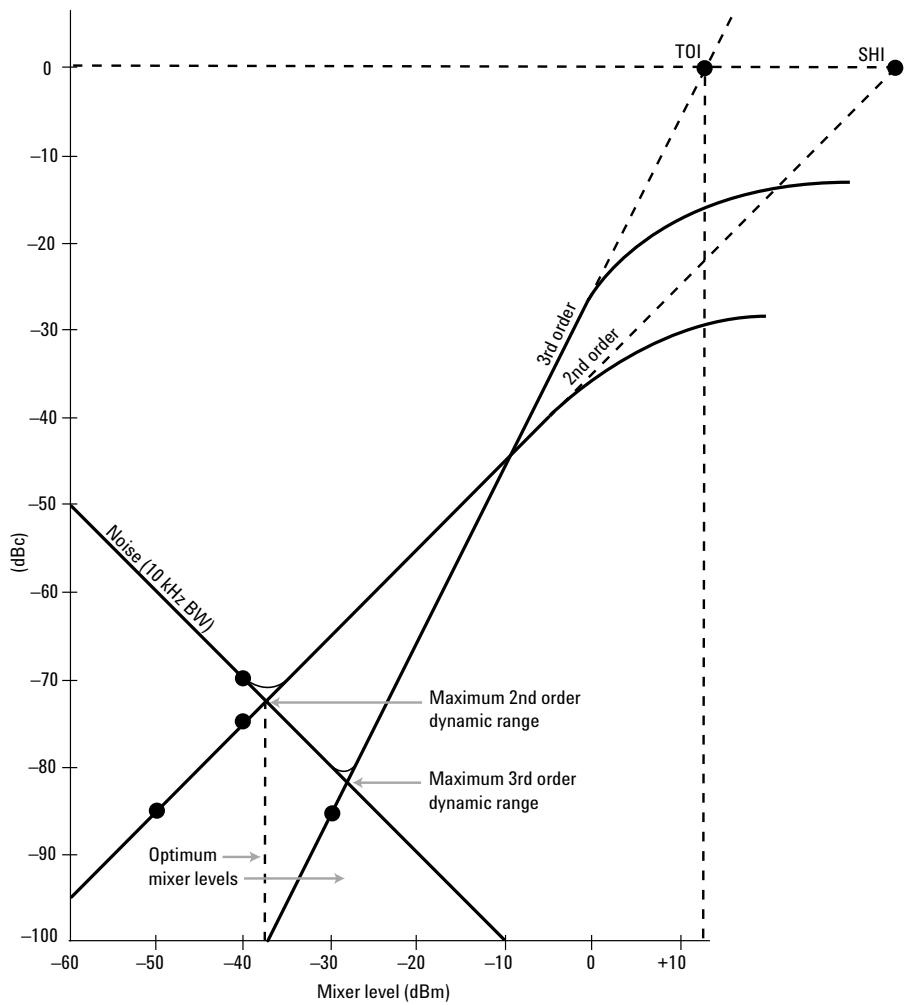
Figure 6-2. Dynamic range versus distortion and noise
