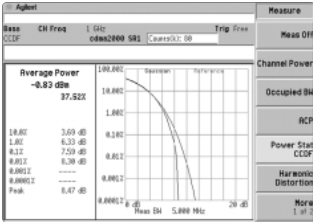
Figure 8-1. CCDF measurement
