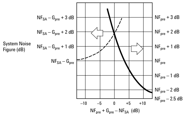
Figure 5-5. System noise figure for sinusoidal signals
