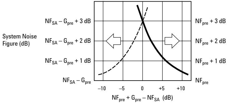
Figure 5-8. System noise figure for noise signals
