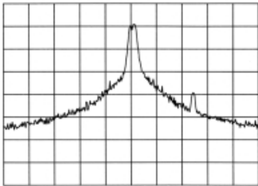
Figure 2-33b. Frequency spectrum of combined signals. Which radio produces the spurious emissions?
