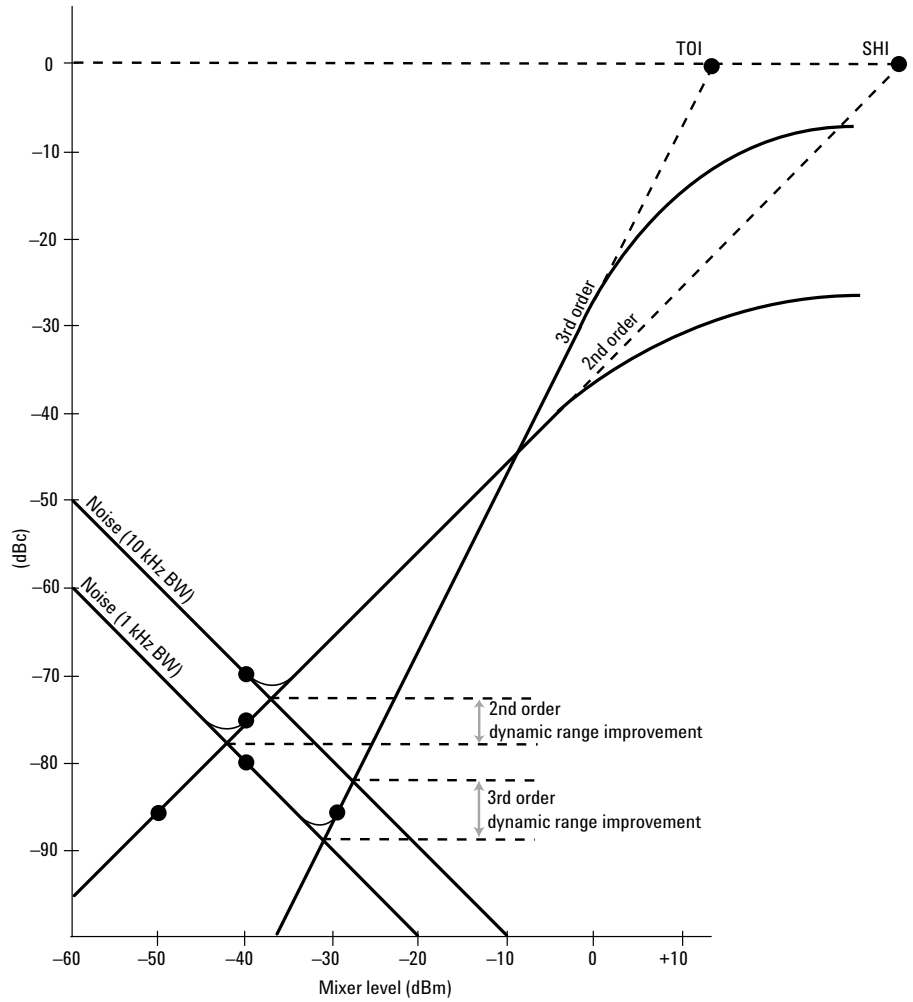
Figure 6-3. Reducing resolution bandwidth improves dynamic range
