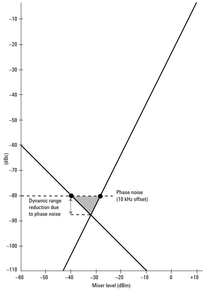
Figure 6-4. Phase noise can limit third-order intermodulation tests
