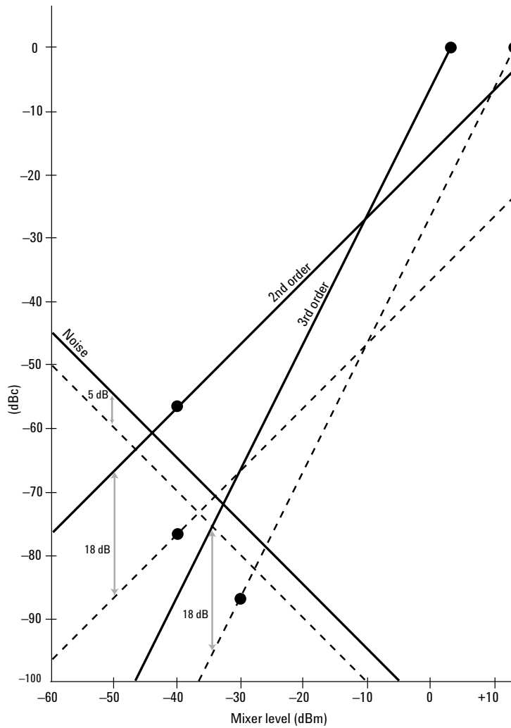
Figure 6-6. Dynamic range for 1.3 dB maximum error
