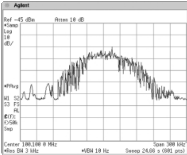
Figure 2-32a. Video filtering
