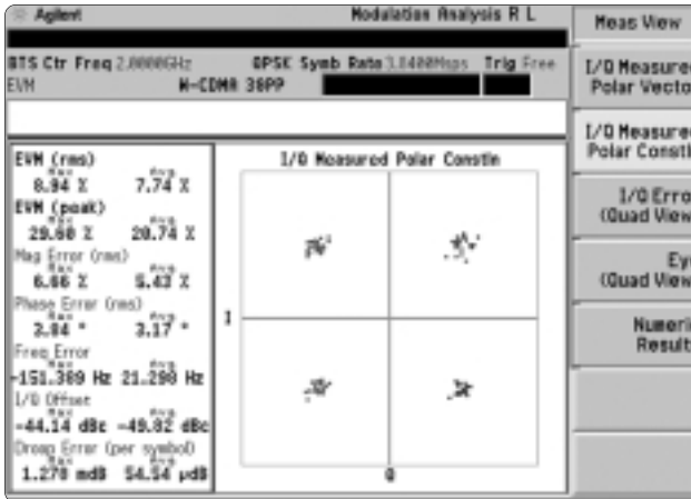
Figure 1-7. Modulation analysis of a QPSK signal measured with a spectrum analyzer
